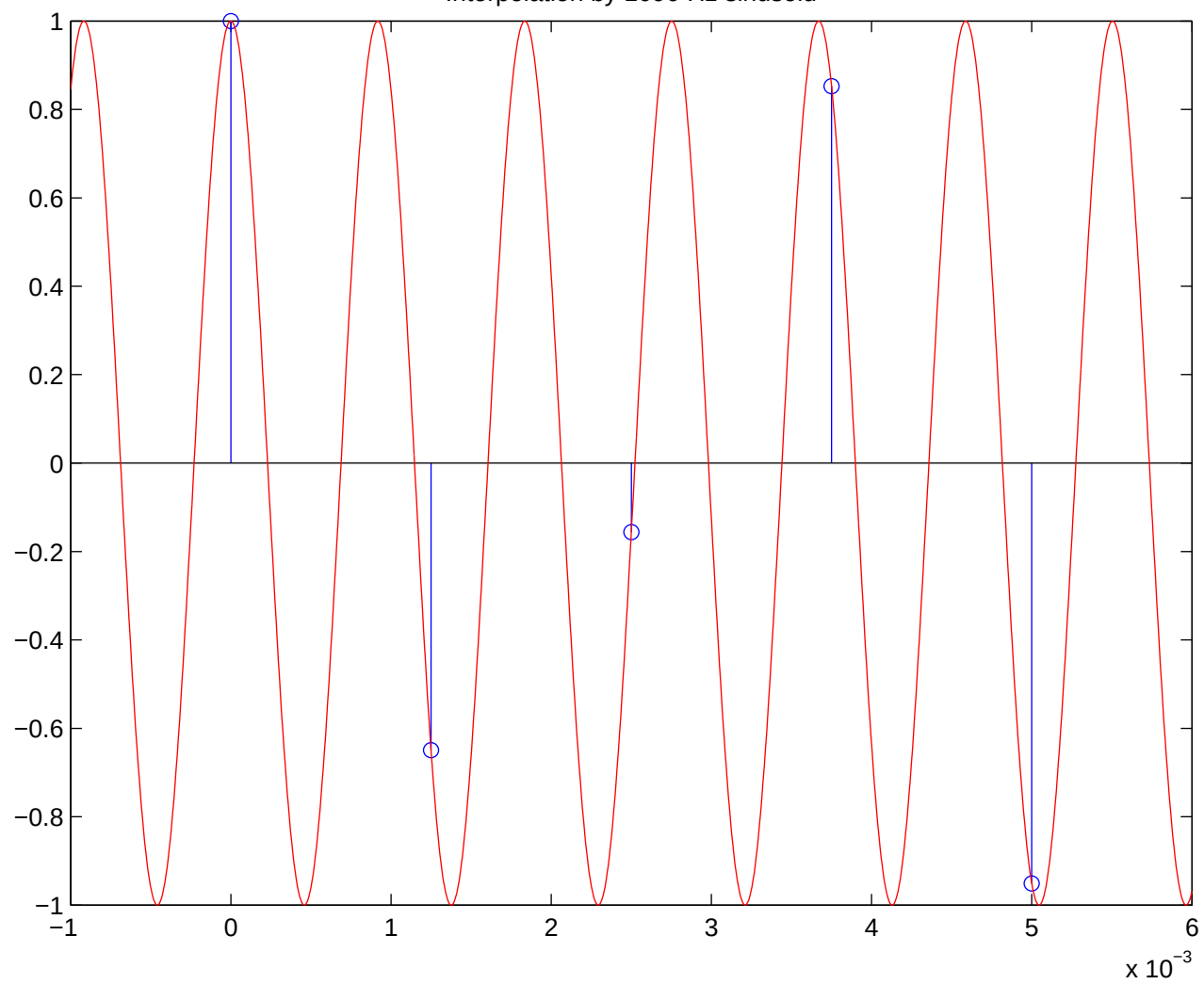
Interpolation by 1090 Hz sinusoid
