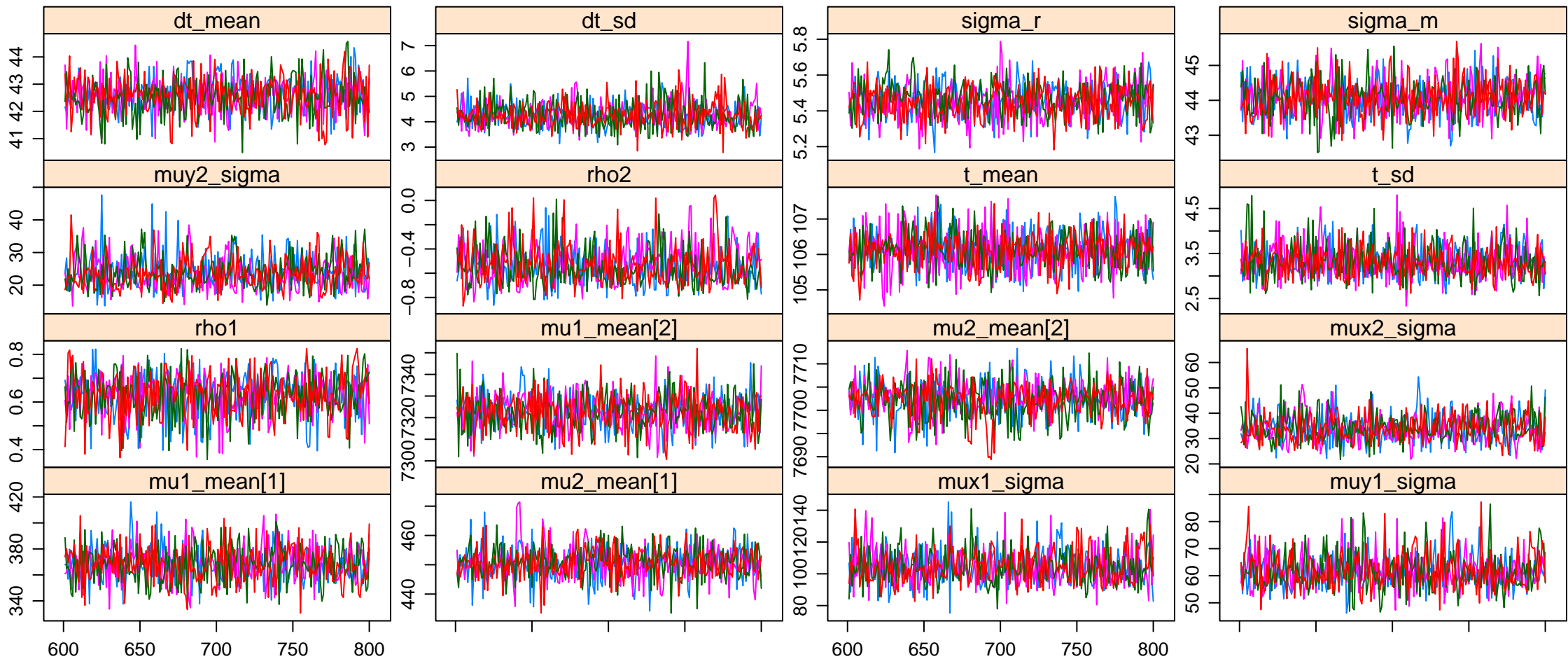
Iteration number
