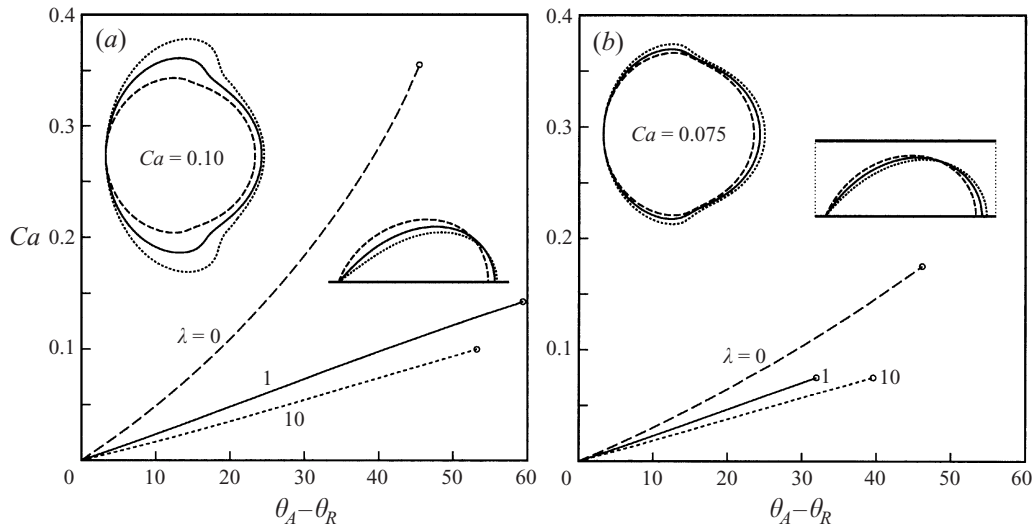
FIGURE 16. Critical capillary number Ca versus hysteresis \theta_A - \theta_R for \theta_A = 90^\circ , for the unconstrained optimal contact line and for several viscosity ratios. (a) The plate spacing is H/h \rightarrow \infty . Also shown are the shapes of the contact line as well as the drop profiles for Ca = 0.10 . (b) As in (a) but for H/h = 1.1 and Ca = 0.075 . Viscosity ratios \lambda : —, 1; ----, 10; ····, 0.
