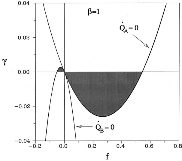
FIG. 8. The contours \dot{Q}_A(f, \gamma) = 0 and \dot{Q}_B(f, \gamma) = 0 are shown, for fixed \beta = 1 . In the shaded regions, there is a net flow of heat out of the colder reservoir; the system then acts as a refrigerator.
