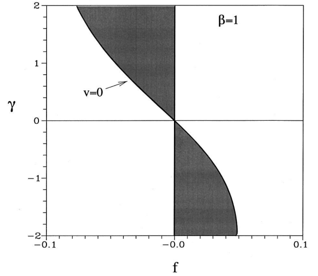
FIG. 7. Contour v(f, \gamma)=0 is shown, for fixed average inverse temperature \beta=1 . The shaded regions are those for which fv > 0 , i.e., for which the system behaves as a heat engine.
