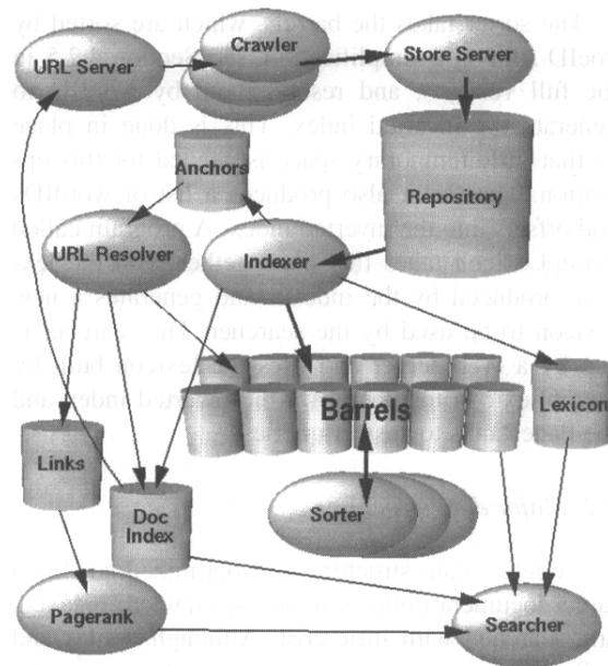
Fig. 1. High level Google architecture.
