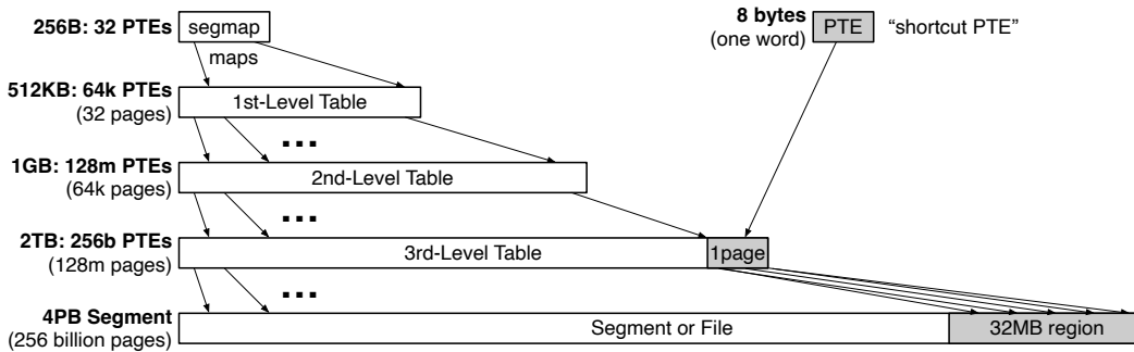
Figure 7: Example segment mapping with 16KB page size and four levels of mapping
