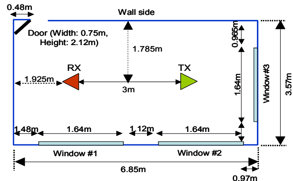
Figure 1: Layout of the residential room
