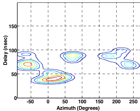
Figure 13: 2-D clusters identified from the simulation (Office NLOS environment, Omni TX)
