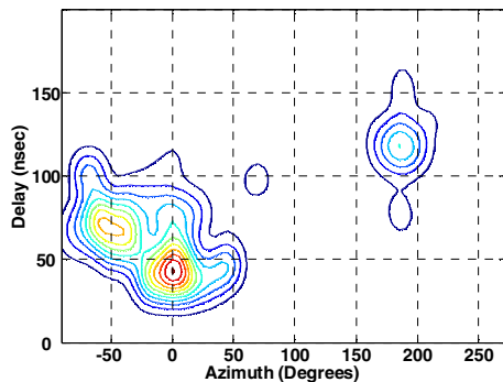
Figure 12: 2-D clusters identified from the experiment (Office NLOS environment, Omni TX)
