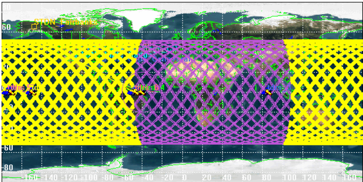
Figure 5.4. ISS Ground track with coverage by just TDRS-8 (highlighted in yellow).
