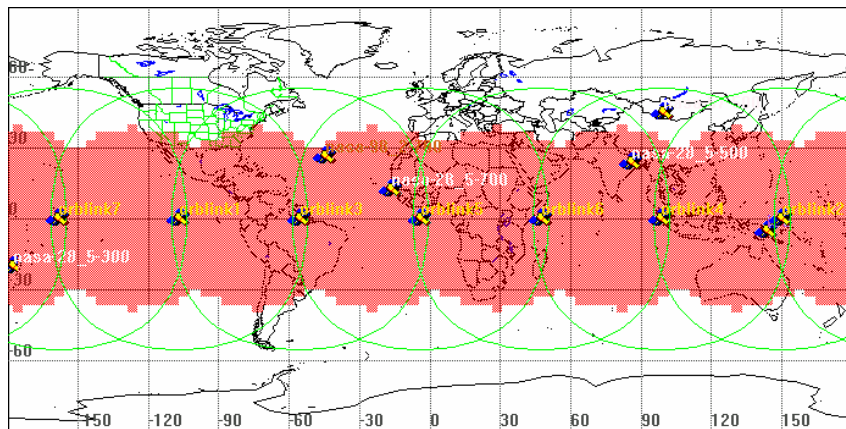
Figure 9c Orblink Static Coverage for mission at 700 km (57.9 %)
