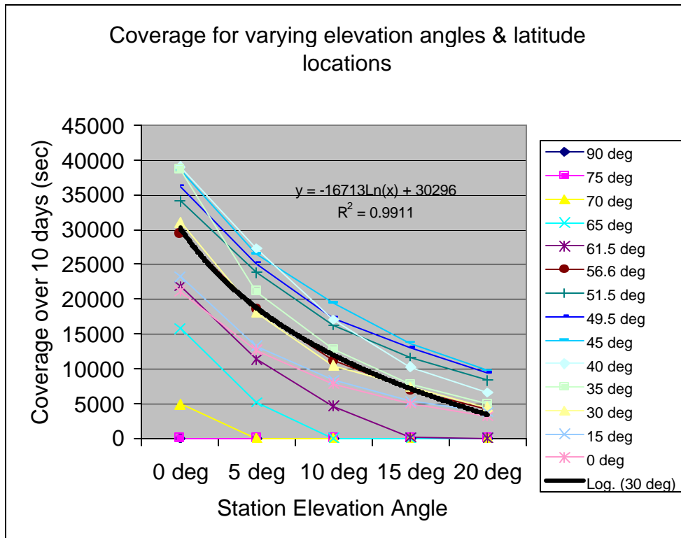
Figure 3.5. Coverage with respect to station minimum elevation angle.
