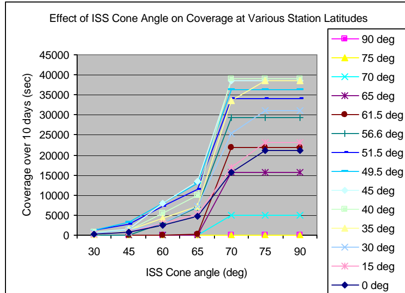
Figure 3.7. Coverage with respect to ISS cone angle.
