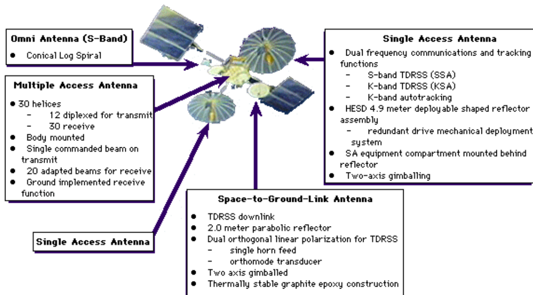
Figure 2.4. Description of TDRS antennas. [5]
