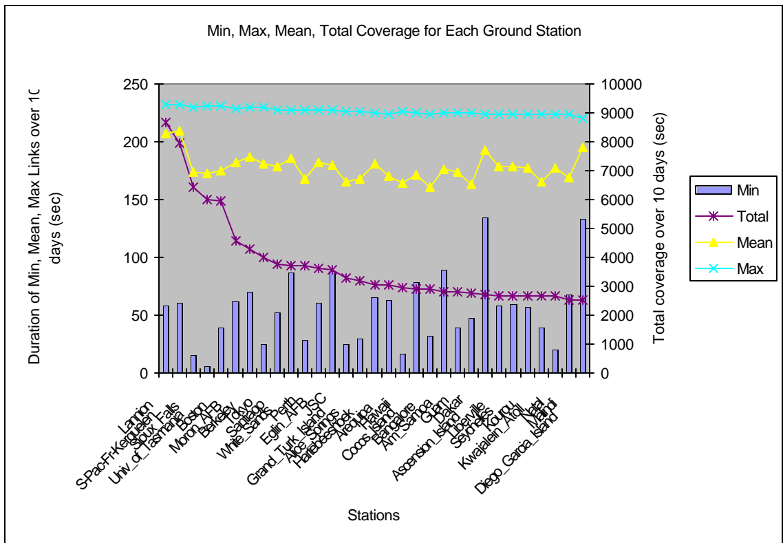
Figure 4.2. Min, max, mean, total coverage for selected stations.
