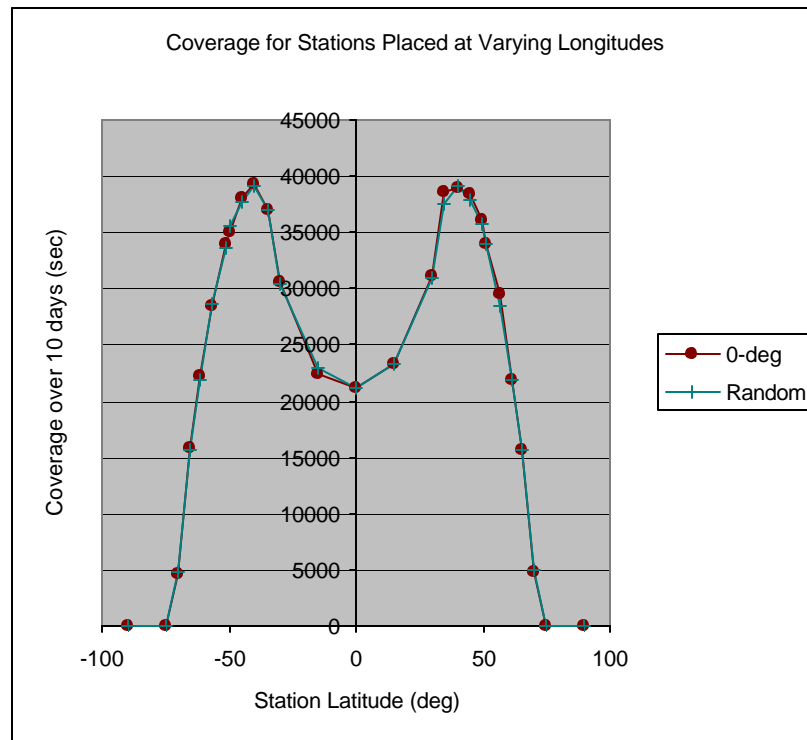
Figure 3.2. Coverage over 10 days for varying station latitude.
