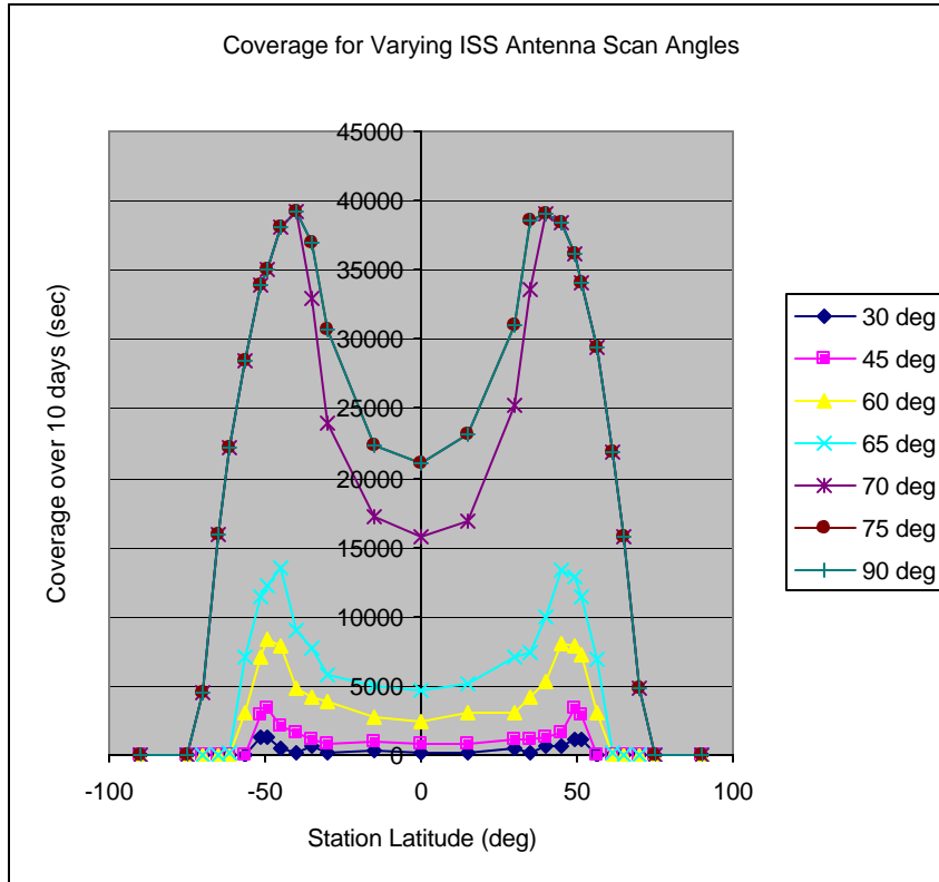
Figure 3.6. Coverage with respect to latitude for varying ISS antenna scan angles.
