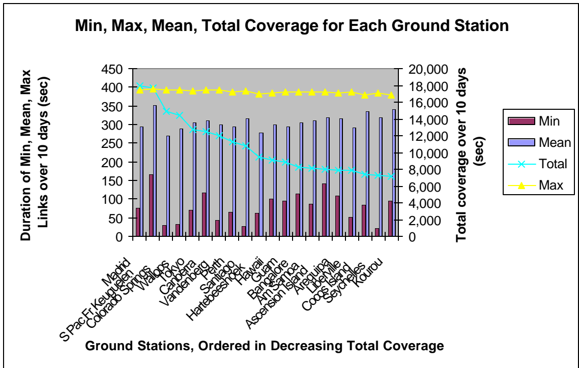
Figure 3.11. Min, Max, Mean Total coverage for selected ground stations.
