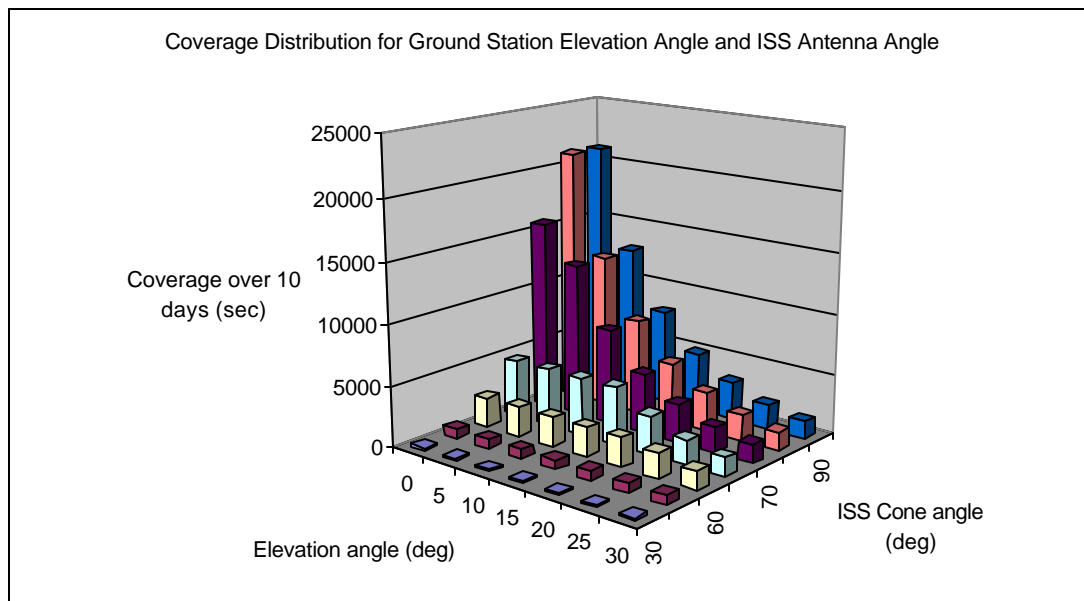
Figure 3.8. Coverage for varying elevation angle and cone angle.
