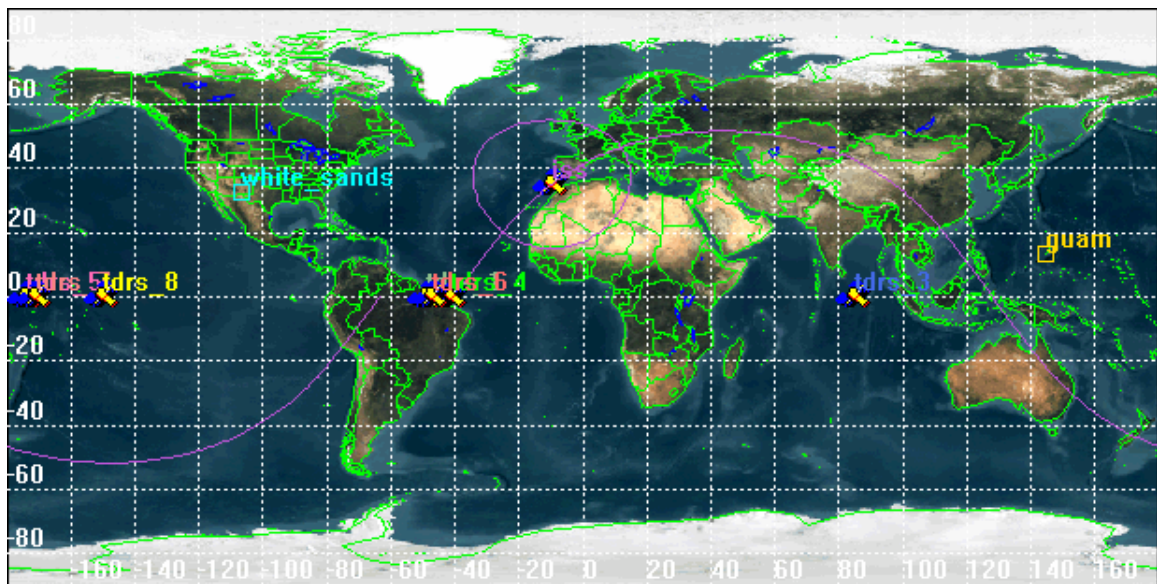
Figure 2.3. NASA TDRSS along with ISS ground track.
