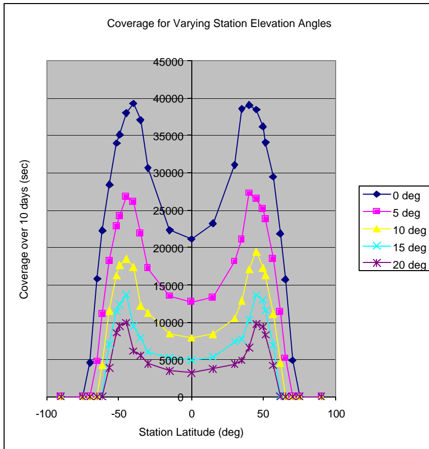
Figure 3.4. Coverage with respect to station latitude for varying min. elevation angles.
