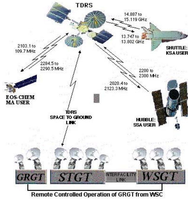
Figure 2.2. Topology of NASA TDRSS.
