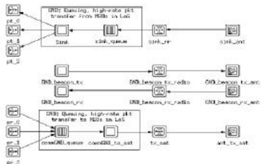
Fig 4. Node model for GND station
