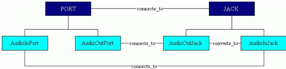
Figure 5.2: Class Relationship in the Port-Jack Ontology
