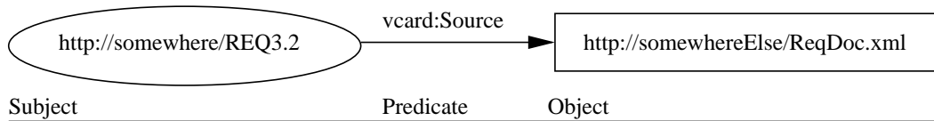
Figure 1.8: RDF Models of an Individual Requirement. In the node and arc diagram, ovals can represent both a subject and object. Rectangular boxes always represent objects. The direction of the arrow is always from the subject to the object of the statement.
