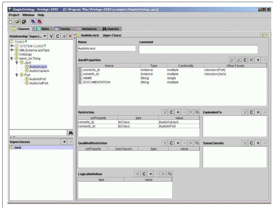
Figure 5.3: A Screenshot of Protégé GUI Illustrating Class Properties of AudioInJack
