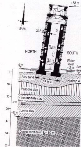
Fig. 2: Soil profile
