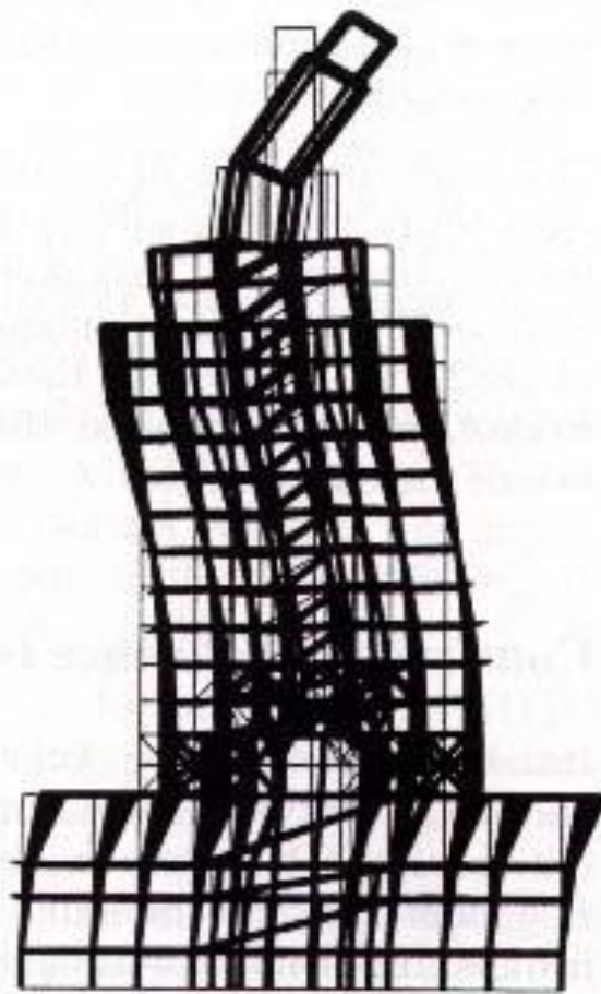
Fixed Base
