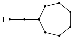
FIGURE 8. A cycle with a tail.
