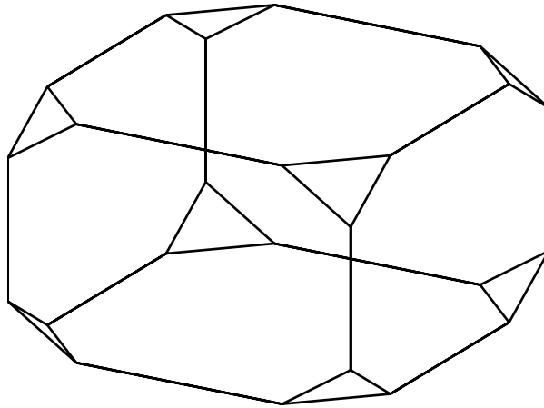
FIGURE 14. A Cayley graph of (\mathbb{Z}_2)^3 \times \mathbb{Z}_3 .
