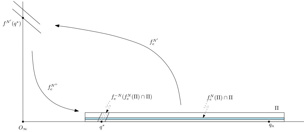
Figure 9: Creation of hyperbolic saddles near the homoclinic point of O_\infty .
