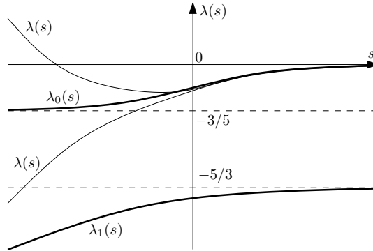
Figure 4: Dynamics of slopes \lambda(s) .
