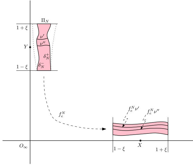
Figure 7: Curves \nu' and \nu'' in Lemma 6.1.
