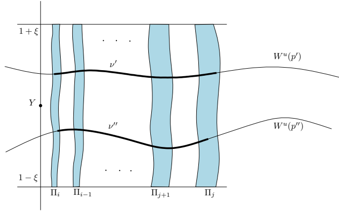
Figure 8: Curves \nu' and \nu'' in Lemma 6.2.
