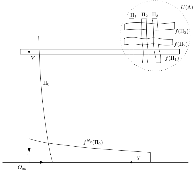
Figure 6: Construction of the set \Lambda^\# .
