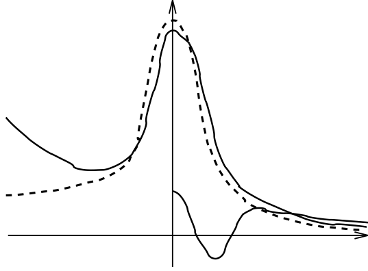
Figure 5: Dynamics of scaled curvature \mu(s) .
