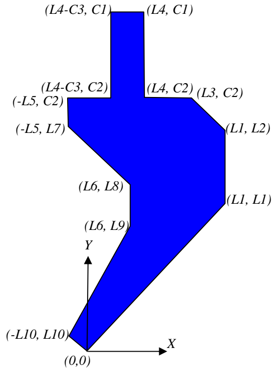
Figure 5: Punch Coordinates in Terms of Punch Parameters
