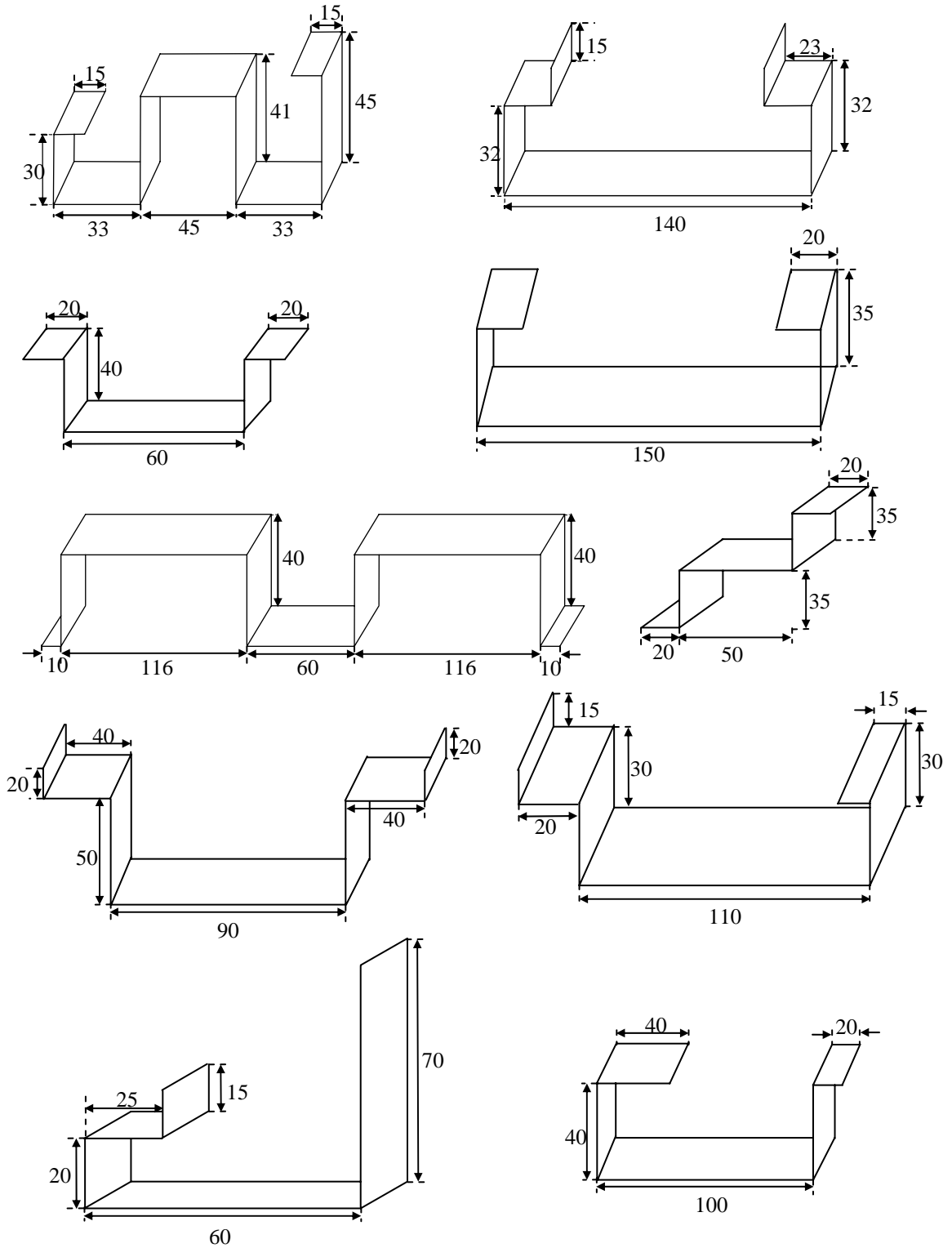
Figure 11: Ten example sheet metal parts
