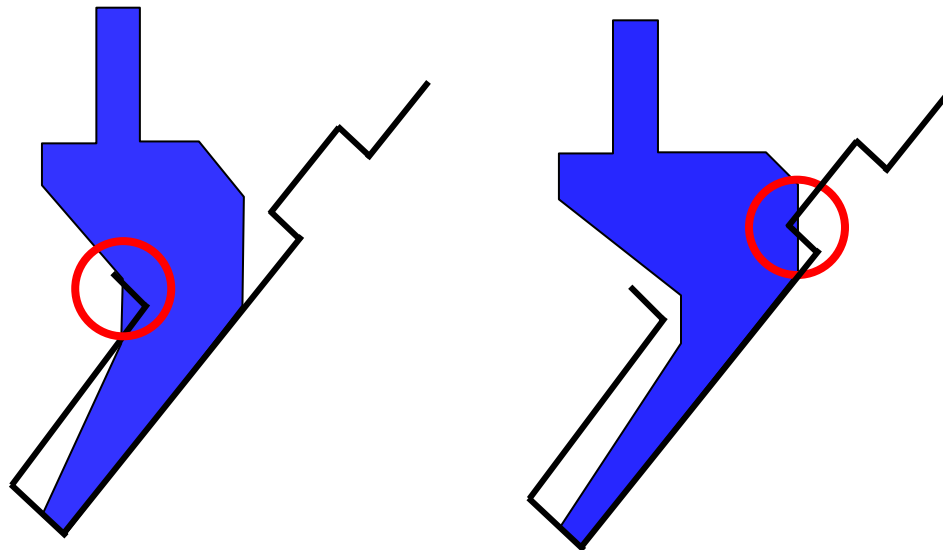
Figure 2: Part tool interference
