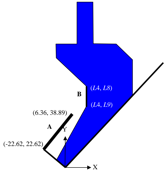
Figure 6: An example of Constraint Generation
