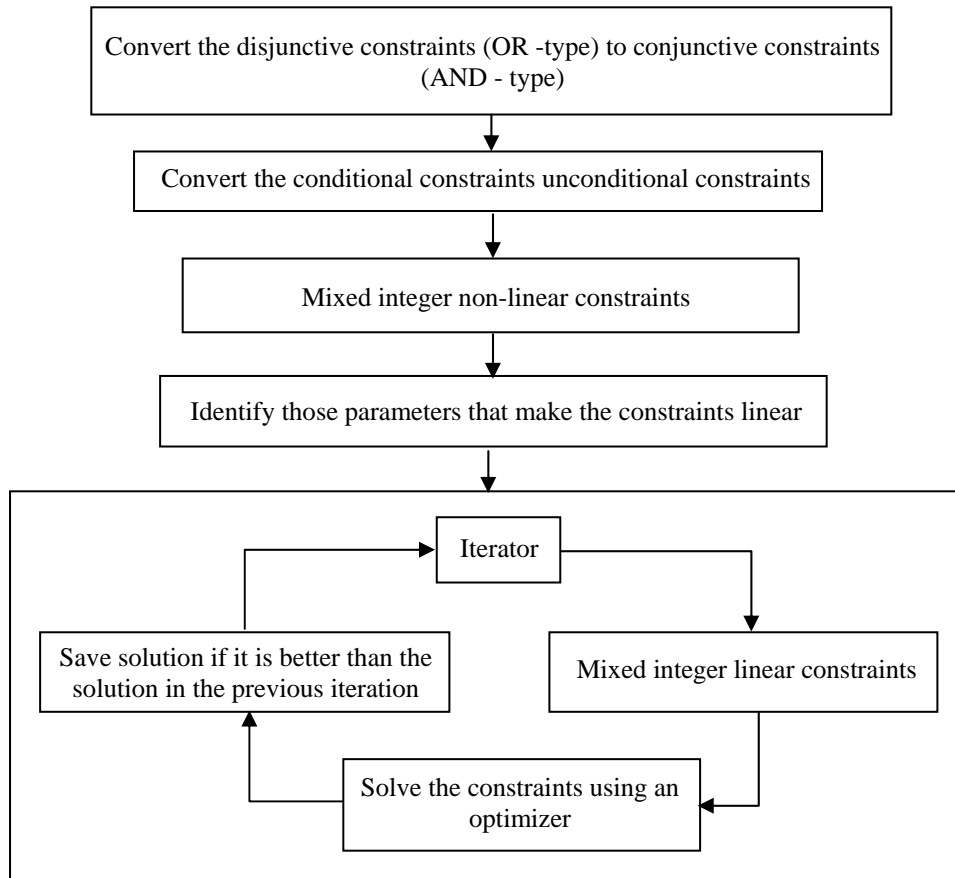
Figure 9: Combined mixed-integer/enumeration formulation
