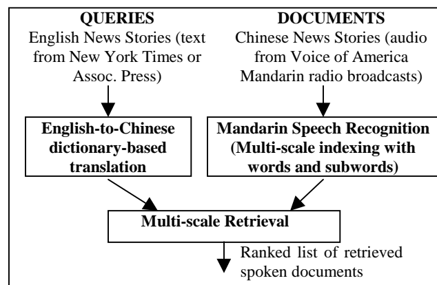
Figure 1. Overview of our English-Chinese cross-lingual spoken document retrieval system. In this task, the query is formed from an entire English news story (text) from the New York Times or Associated Press. The spoken documents are Mandarin news stories (audio) from Voice of America news broadcasts. Multi-scale retrieval of the spoken documents is evaluated based on the relevance of the ranked list of spoken documents retrieved for each query.
