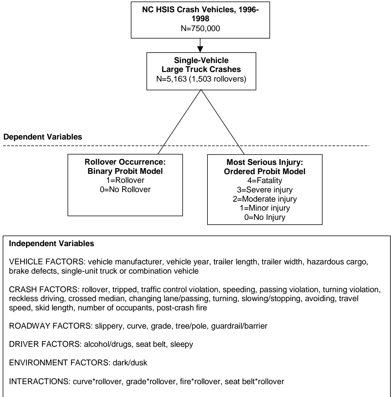
FIGURE 2 Data structure
